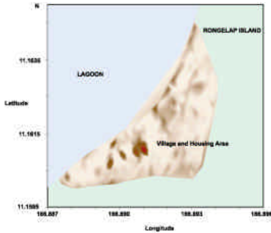
Figure 4b. ^{137}\text{Cs} dose rates after addition of coral fill (Rongelap Island, April 2001).
