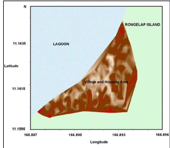
Figure 4a. ^{137}\text{Cs} dose rates after removal of surface soil (Rongelap Island, May 2000).
